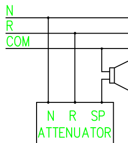
3-WIRE CONNECTION
