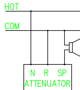
2-WIRE CONNECTION
